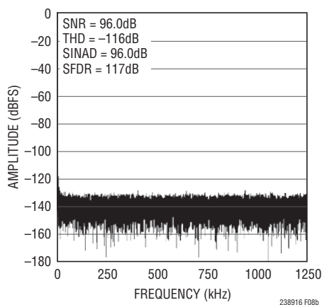
Figure 8b. 32k Point FFT f_{\text{SAMPL}} = 2.5\text{Msps} , f_{\text{IN}} = 2\text{kHz} , for Circuit Shown in Figure 8a
